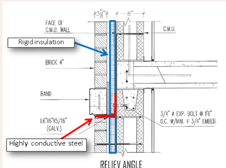
Wall construction utilizing shelf angle
